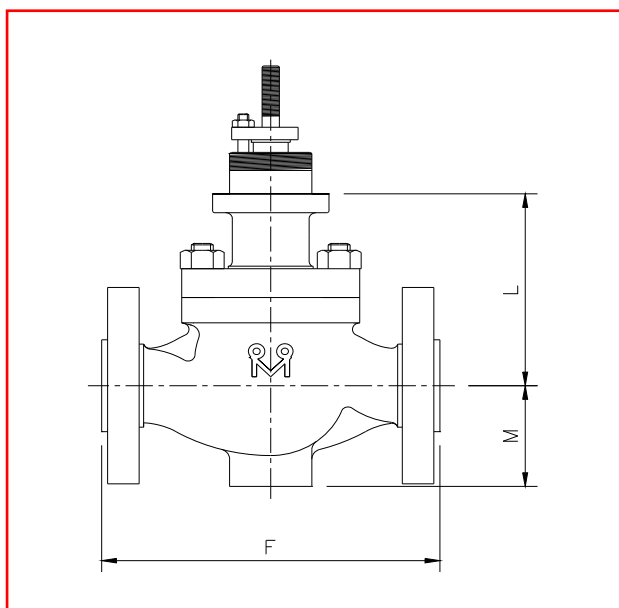
Figure 9. Series 07 dimensions
