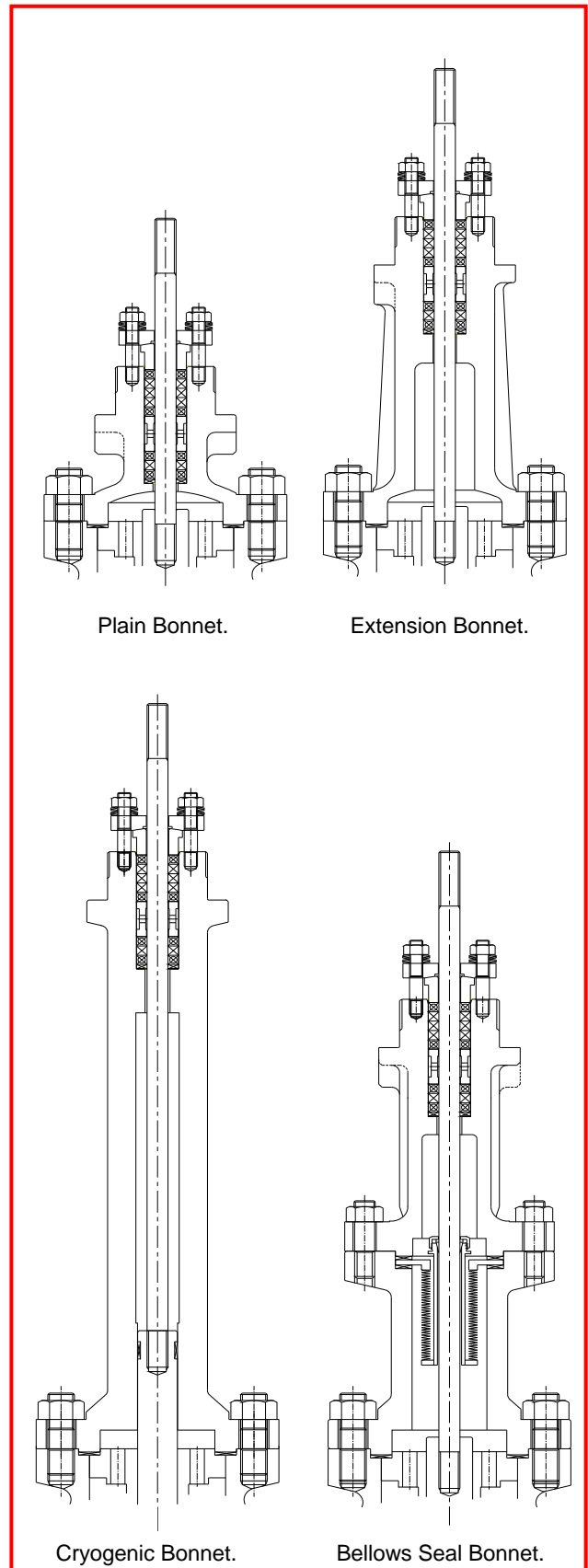
Figure 7. Bonnet design option
